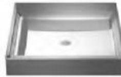
description: SHOWER PAN model: 3636CPAN material: COMPOSITE / SMC size: 36"W x 36"D x 6"H
